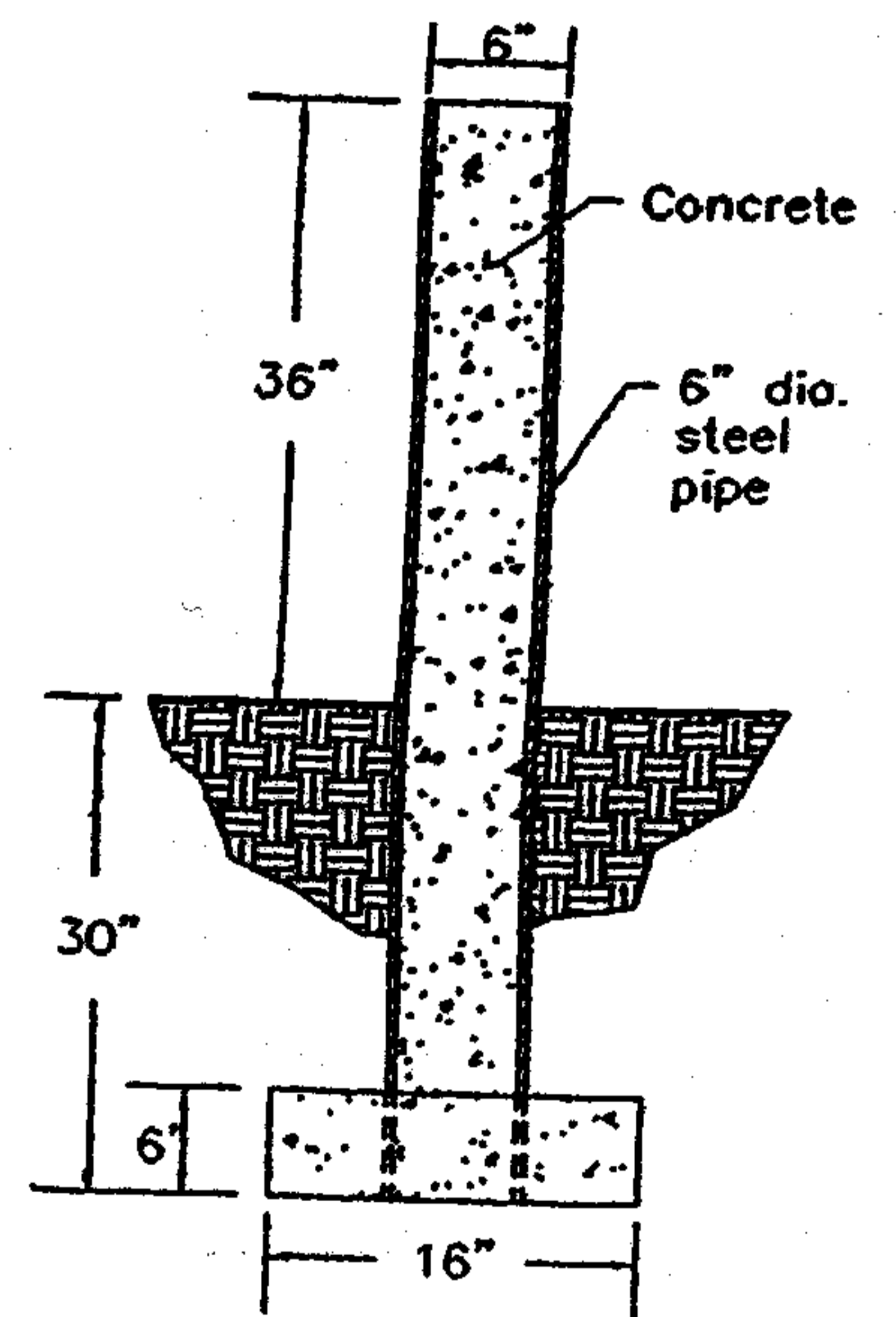
BOLLARD DETAIL
