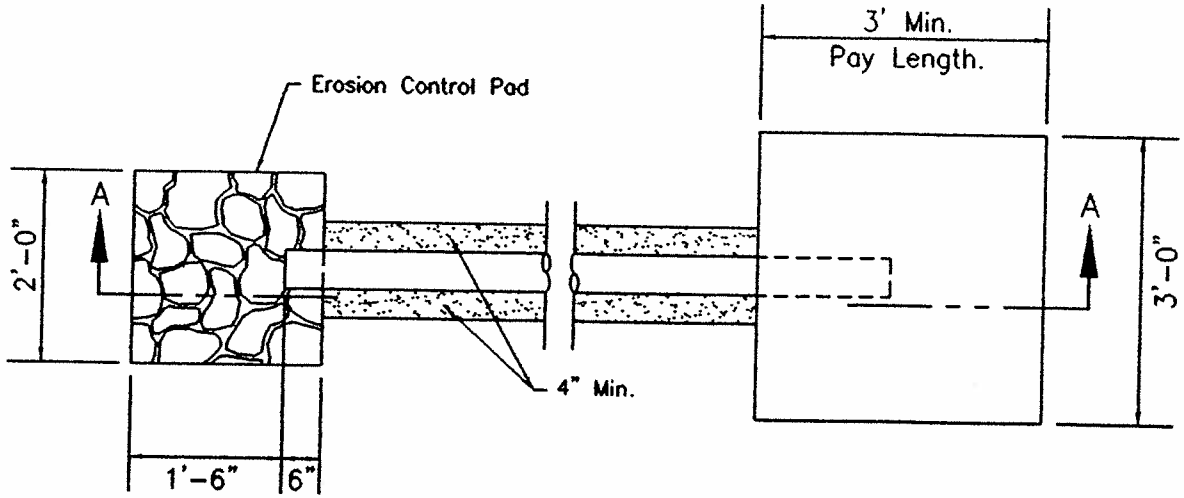
PLAN
