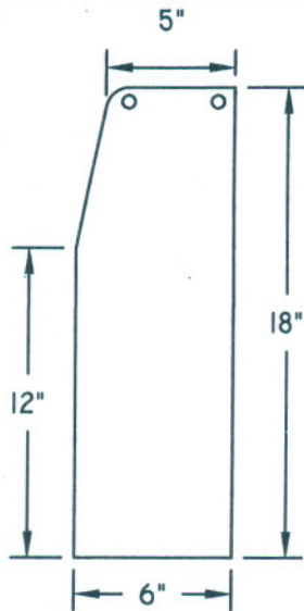
STD. FULL DIVISION PLATE
